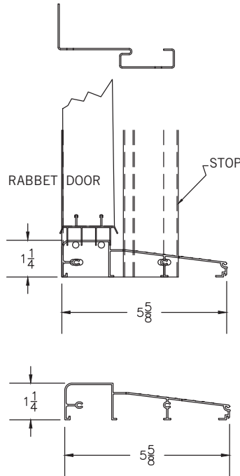
5-5/8" ADA SADDLE SILL
