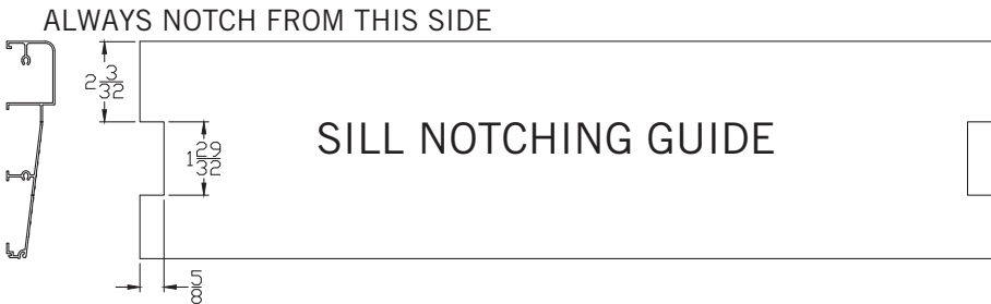
5-5/8" ADA SADDLE SILL
